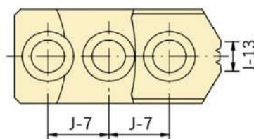
排齒詳圖 Drawing of Serration
