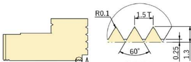
排齒詳圖 Drawing of Serration
