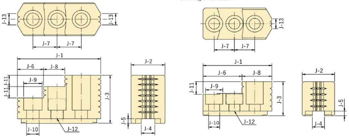
排齒詳圖 Drawing of Serration
